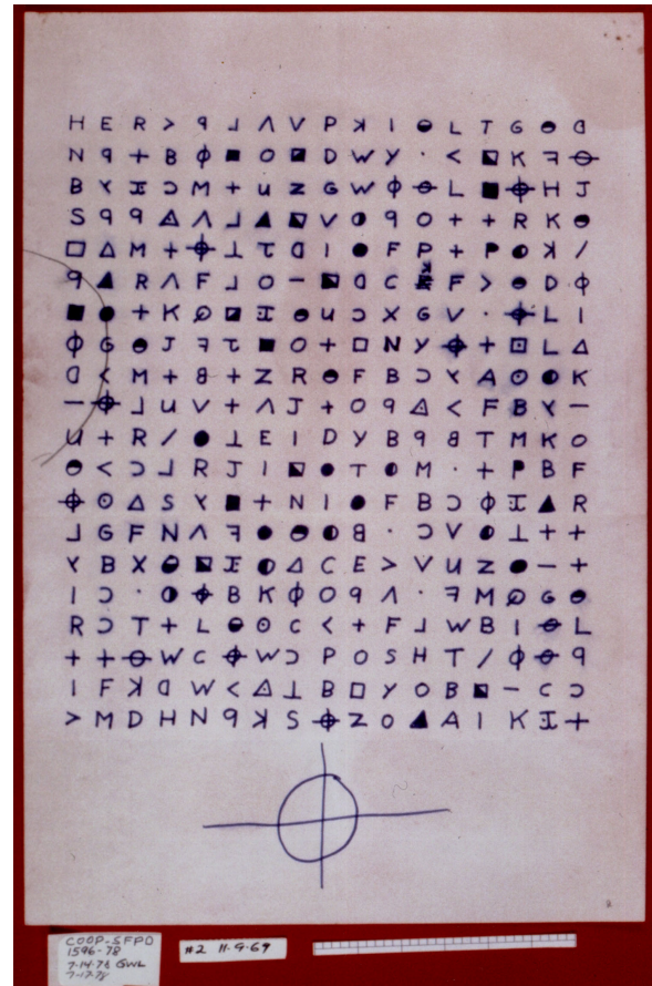
Figure 1: Zodiac-340 ciphertext. 1
