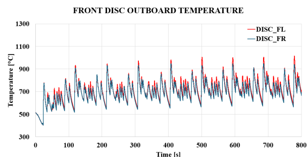
Figure 9: Front discs outboard temperature in a driving simulator session
