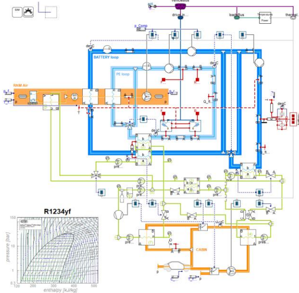
Figure 16. Thermal management system
