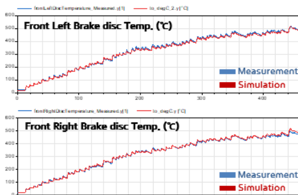
Figure 7. Comparison of the brake thermal model with experimental results
