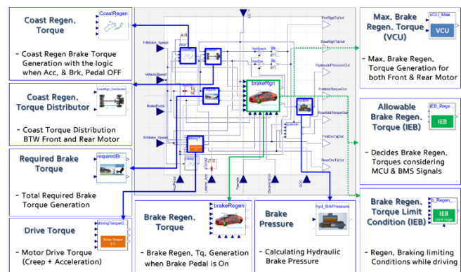
Figure 3. Vehicle Controller Model built for Electric AWD Durability Scenarios
