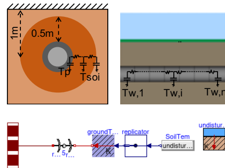
Figure 4. Representative diagram of the radial heat transfer between the distribution pipe T_p and the ground T_{soil} (left). Axial discretization of the pipe water volumes T_{w,i} (right). Below is a diagram view of the ground coupling model.
